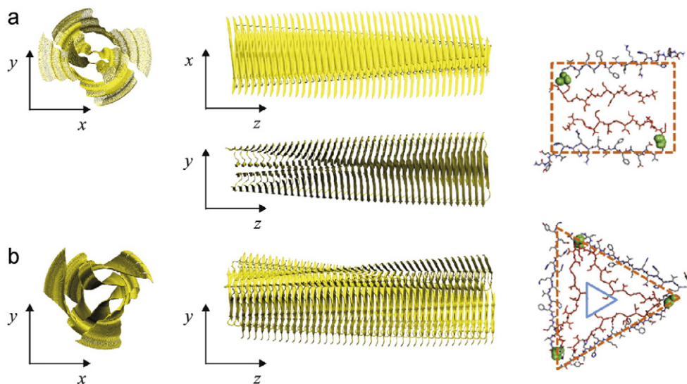
Fig. 11. Structures of a. twofold and b. threefold symmetric assemblies of Aβ(1–40) amyloid fibrils. Reprinted with permission from Xu et al. [86], Biophys. J. 2010, 98.
