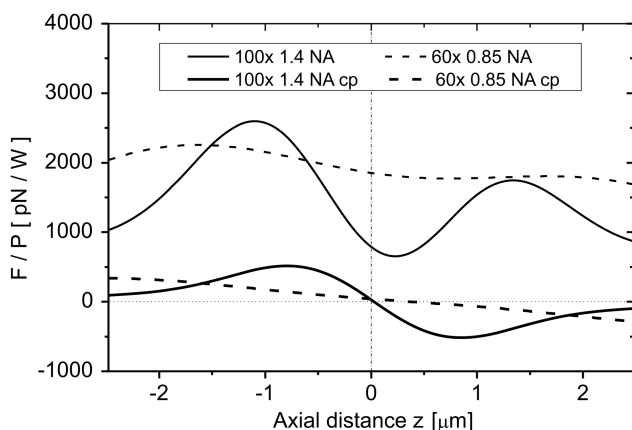
Fig. 8. Calculated axial force (assuming no spherical aberrations) for a 1.1 \mu\text{m} diameter \text{TiO}_2 particle ( n = 2.4 ) in ethanol ( n = 1.36 ) for high-NA objectives (100 \times , 1.4 NA; solid curves) and low-NA objectives (60 \times , 0.85 NA; dashed curves). There is no stable trapping position for the single-beam traps. In the counterpropagating (cp) beams, the axial stiffness \kappa_z at the stable trapping position is 1043 \text{ pN}/(\mu\text{m} \times W) (1.4 NA) and 103 \text{ pN}/(\mu\text{m} \times W) (0.85 NA).
