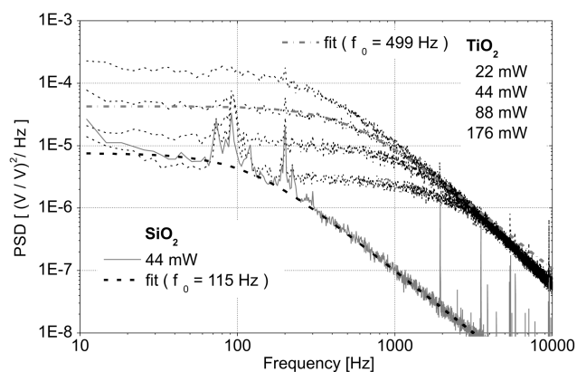
Fig. 3. PSD curves of the normalized signal for a \text{SiO}_2 (gray solid curve, diameter 1.4\text{ }\mu\text{m} ) and a \text{TiO}_2 (black dotted curves, 1.1\text{ }\mu\text{m} ) particle in ethanol for given laser powers inside the counterpropagating trap. For clarity only one curve is shown for \text{SiO}_2 . Lorentzian fits (dashed curves) are plotted for the 44 mW curves, with f_0 at 115 Hz ( \text{SiO}_2 ) and 499 Hz ( \text{TiO}_2 ). Highest laser powers result in lowest plateau values.
