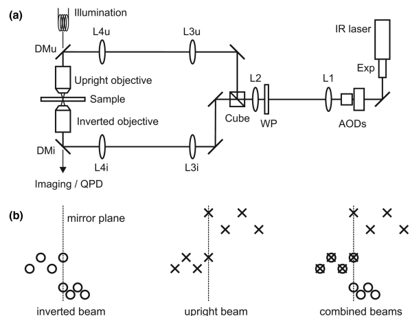
Fig. 1. Schematics of (a) the optical tweezers setup and (b) the counterpropagating traps scanned with one pair of AODs. A pattern of inverted beam traps ( \circ ) is a mirror image of the pattern of upright beam traps ( \times ) with the mirror plane top-to-bottom in the image. In addition, the magnification between the inverted and the upright beam path might differ. By adding a mirrored and appropriately scaled pattern to the original traps, counterpropagating traps ( \otimes ) can be created for which the position of each trap can be chosen arbitrarily.
