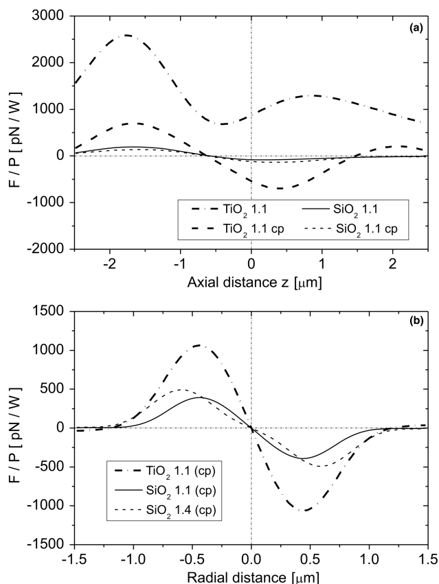
Fig. 4. Calculations of the force per 1 W laser power for 1.1\ \mu\text{m} diameter \text{TiO}_2 ( n = 2.4 ) and \text{SiO}_2 ( n = 1.45 ) particles in ethanol ( n = 1.36 ) in Gaussian single and cp traps using 100\times , 1.4\ \text{NA} , oil immersion objectives. Spherical aberrations are accounted for. (a) Axial force, with z as the offset of the particle from the focal plane of one objective and (b) radial force at the trapping plane for 1.4\ \mu\text{m} \text{SiO}_2 ( z = -0.628\ \mu\text{m} ) as a function of the distance to the optical axis. In addition, the curve for 1.4\ \mu\text{m} \text{SiO}_2 is shown.
