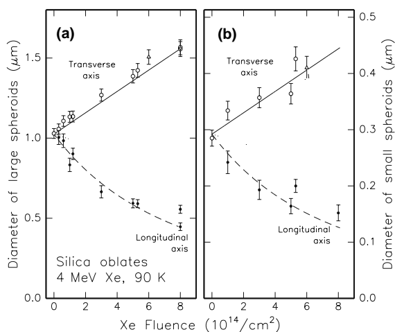
Fig. 2. Transverse and longitudinal diameters of large (a) and small (b) silica spheres as a function of 4 MeV Xe 4+ irradiation fluence. All irradiations were performed at 90 K. The line drawn through the data for the transverse axis is a linear fit, the dashed line is a calculation derived from the drawn line assuming the particle volume remains constant with fluence.
