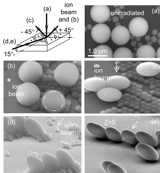
Fig. 1. SEM images of silica (a)–(d) and ZnS (e) particles on a Si substrate: (a) top view ( 0^\circ tilt) of as-deposited silica spheres with two different diameters; (b)–(d) silica spheroids after 4 MeV Xe irradiation to a fluence of 3 \times 10^{14} \text{cm}^{-2} , under an angle of +45^\circ , at 90 K. The ion beam direction and the different viewing angles are indicated in the schematic inset for each image; (e) ZnS microspheres irradiated with 5 \times 10^{14} \text{Xe}/\text{cm}^2 under an angle of 45^\circ at 90 K. All images are taken at the same magnification.
